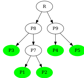
Figure 13: Plot of the five-population graph on which to add the P6 population with the add.leaf function
