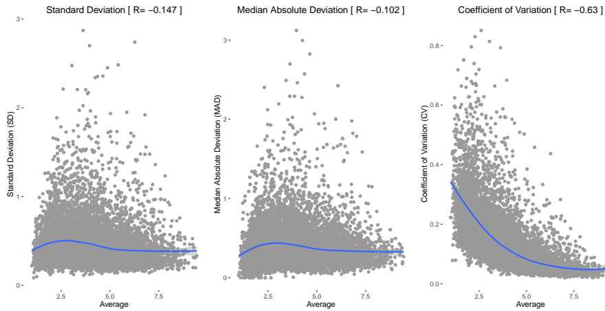
Figure 3: Relationships between SD, MAD, CV with the mean for the two sample case.
