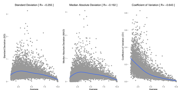
Figure 2: Relationships between SD, MAD, CV with the mean for the one sample case.
