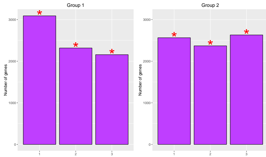
Figure 7: Distribution counts of the standard deviation of ESC (group 1) and IPS (group 2) for the all genes in the Bock data set.
