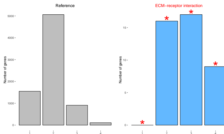
Figure 4: Histogram of the "ECM-receptor interaction" pathway and the reference counts.
