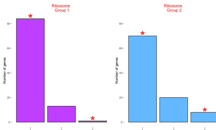
Figure 6: Distribution counts of the standard deviation of ESC (group 1) and IPS (group 2) for the "Ribosome" pathway.
