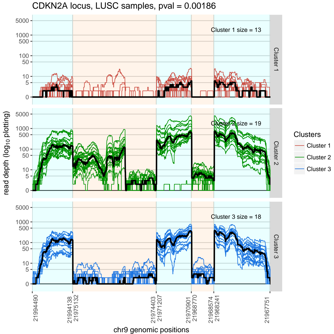
Figure 3: Graphical output from SFfigure for lplots = 3 .
