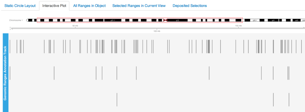
Figure 6: Interactive Plot
