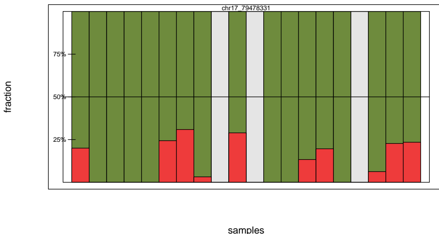
Figure 3: A barplot with type='fraction' Each bar represents one sample and by default the most expressed allele over all samples is on the top, here in green. The black line denotes 1:1 expression of the alleles.
