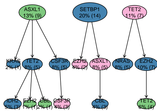
MST Prim – aCML data
