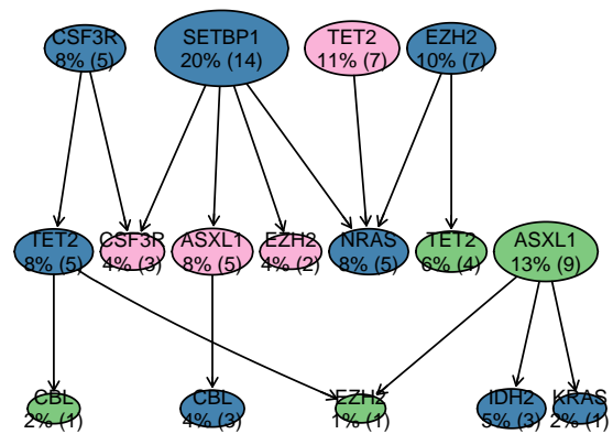
Figure 12: aCML data processed model by algorithms to extract models from individual patients, we show the output of CAPRESE, and all algorithms based on Minimum Spanning Trees (Edmonds, Chow Liu and Prim)
