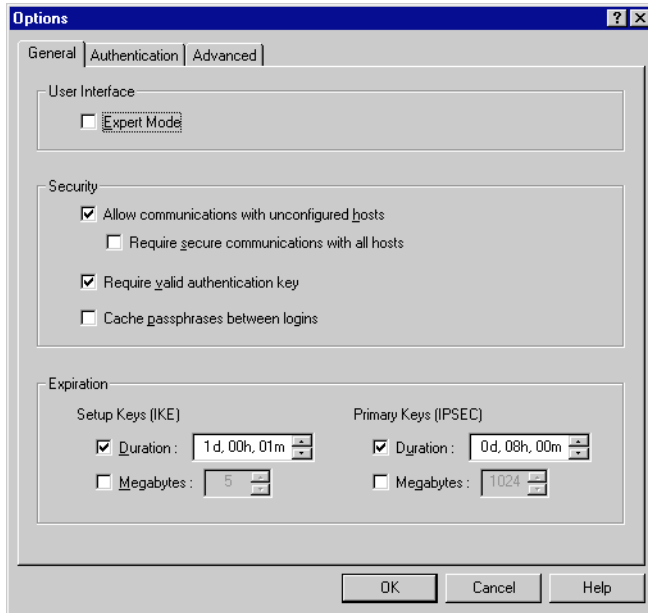
Figure 7-10. The General Panel
