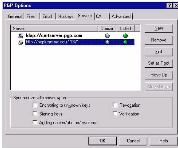
Figure 6-14. PGP Options dialog box (Server panel)
