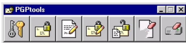
Figure 2-3. PGPtools
