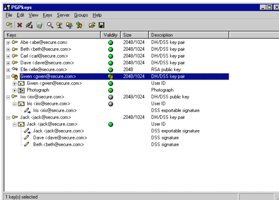
Figure 2-1. PGPkeys
