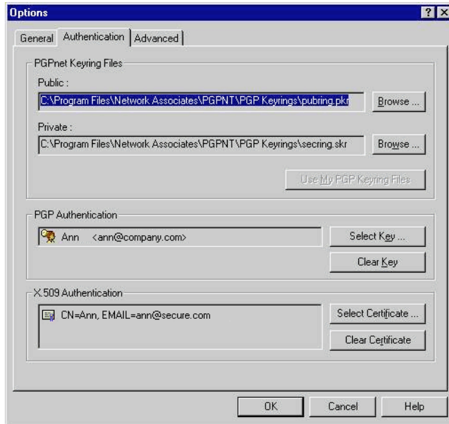
Figure 7-2. The Authentication Panel
