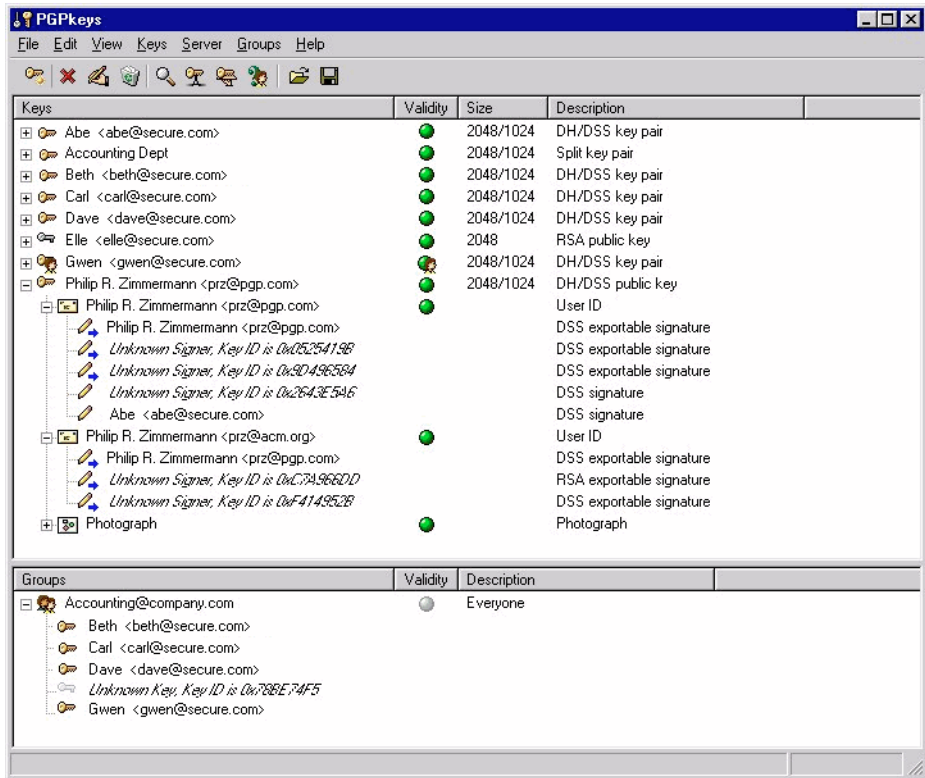
Figure 4-4. PGPkeys with Groups window
