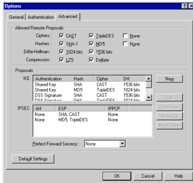
Figure 7-12. The Advanced Panel
