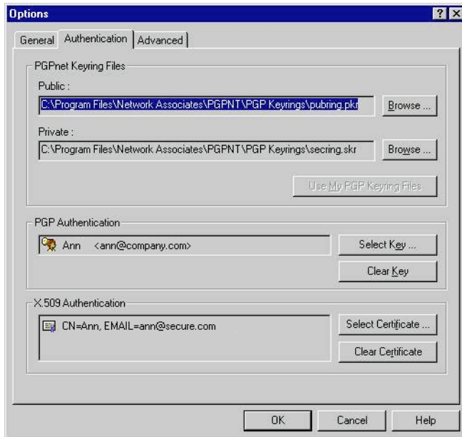
Figure 7-11. The Authentication Panel
