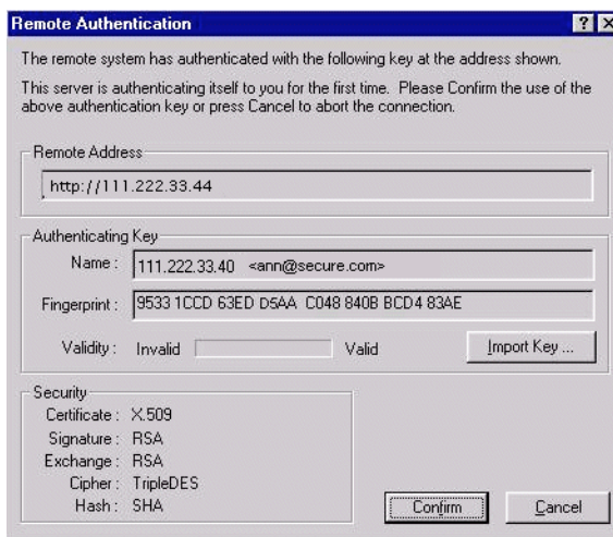
Figure 3-14. Remote Authentication dialog box
