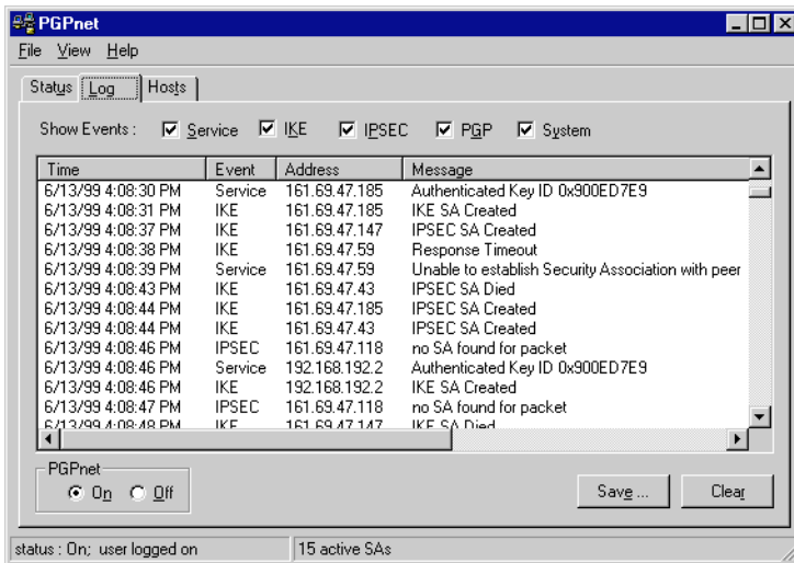
Figure 7-5. The Log Panel
