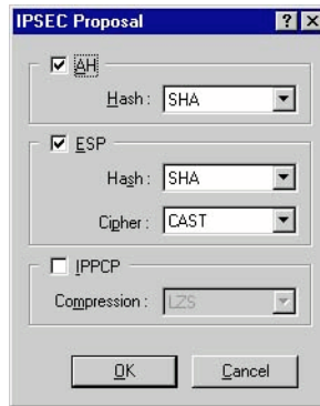
Figure 7-14. IPsec Dialog
