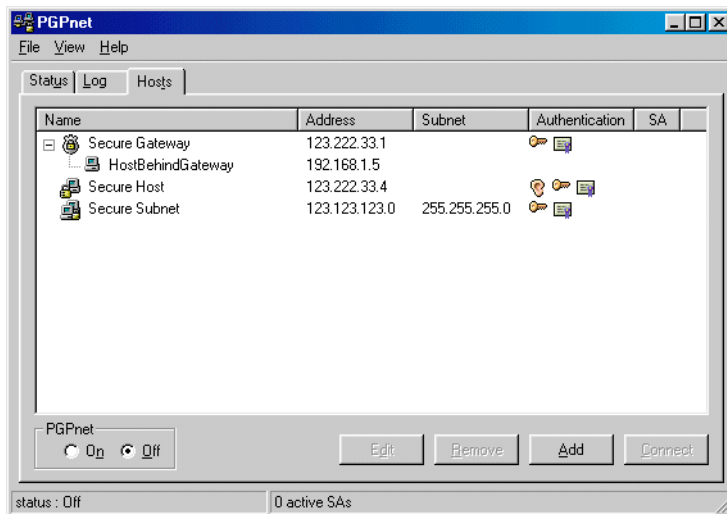
Figure 7-6. The Hosts Panel
