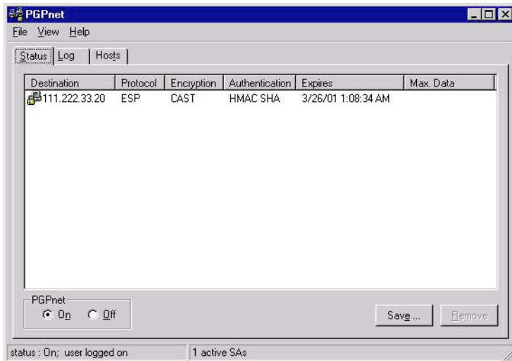
Figure 7-3. PGPnet window
