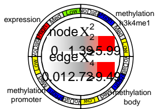
Network built around DPYSL4:NRP1:SEMA3A Chi-square P-value= 0.004
