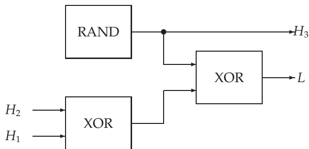
Figure 8.4: Insecure composition of secure systems with feedback
