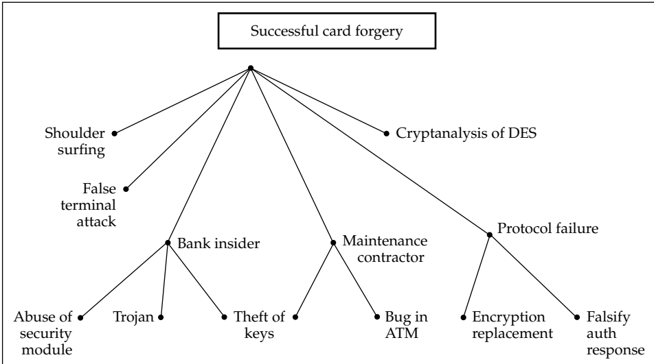
Figure 25.4: A threat tree
